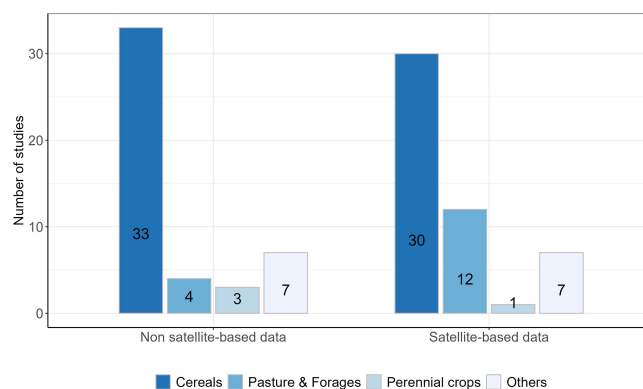
Figure 4. Use of satellite data for different types of insured crops. Crops are categorized into four major groups: cereals, pasture and forages, perennial crops, and others (such as vegetables, oilseed crops, fruits, nuts, etc.).
