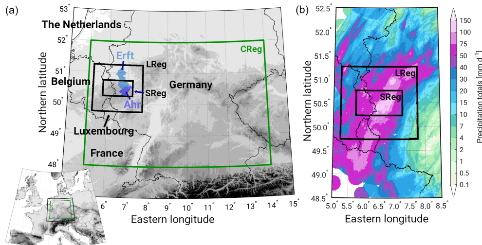
Figure 1. (a) Overview map of central and western Europe (bottom left) with a zoom-in on the region of interest and (b) 24 h precipitation totals of 14 July 2021 based on RADOLAN (cf. Part 1). Two regions (LReg, SReg; black rectangles) covering the main precipitation area and the affected river catchments of the Ahr (dark blue) and the Erft (light blue) are defined to derive specific event characteristics (e.g., spatial means). Analyses in a statistical and climatological context are performed over the greater central Germany region (CReg, green box). Topographic data (gray) were provided by NOAA National Geophysical Data Center (Amante and Eakins, 2008).
