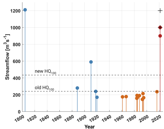
Figure 7. Time series of selected flood peaks at gauge Altenahr (Ahr). The blue dots are reconstructions (modified from Roggenkamp and Herget, 2022); the orange dots are the 10 largest floods in the gauge recordings (starting 1946), provided by the water authority of Rhineland-Palatinate; the red dots indicate the range of the 2021 flood peak estimated by the water authority of Rhineland-Palatinate; and the black crosses indicate the range of the 2021 flood peak estimated by Roggenkamp and Herget (2022) based on gauge recordings and reconstructions. The two dashed lines indicate the official HQ_{100} estimates using only instrumental recordings (since 1946; old HQ_{100} = 241\text{ m}^3\text{ s}^{-1} ) and a new approach including historical sources (new HQ_{100} = 434\text{ m}^3\text{ s}^{-1} ).
