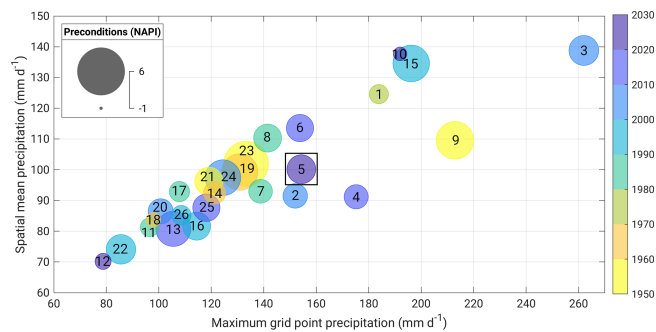
Figure 3. Bubble plot of the most extreme precipitation events in Germany according to the HPE_{crit} based on daily HYRAS-DE data (1951 to 2021). The maximum 24 h grid point intensity within the HPE_{crit} area A is given on the x axis; the y axis represents the spatially averaged 24 h precipitation over A . The size of the bubbles (small inset legend at the top left) represents the preconditions using the normalized antecedent precipitation index (NAPI, see the Supplement), while the color indicates the decade of occurrence. The numbers give the ranking according to the HPE_{crit} (see Table S2). The July 2021 event (ranked fifth) is marked with a rectangle.
